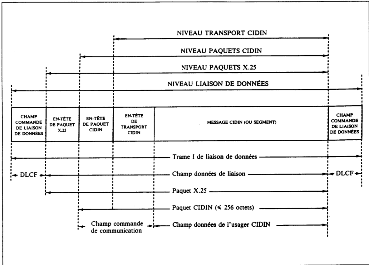
Figure 8-2. Terminologie CIDIN
