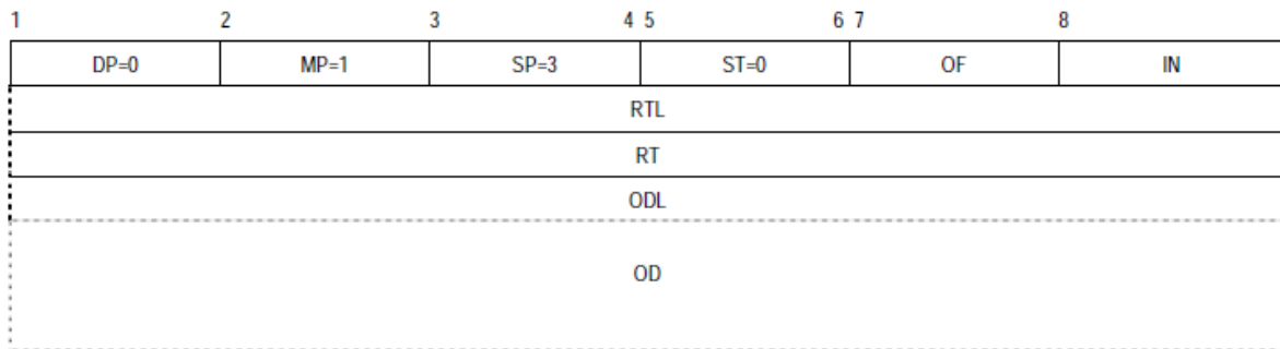
Figure 5-19. Paquet ROUTE
