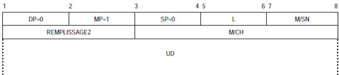
Figure 5-22. Paquet MSP LONG
