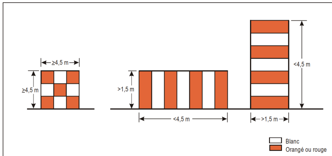
Figure 6-1. Marquages types
