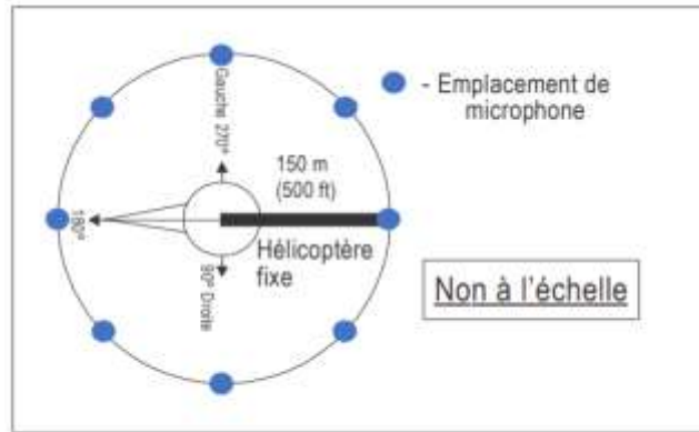
Figure H-2. Configuration circulaire
